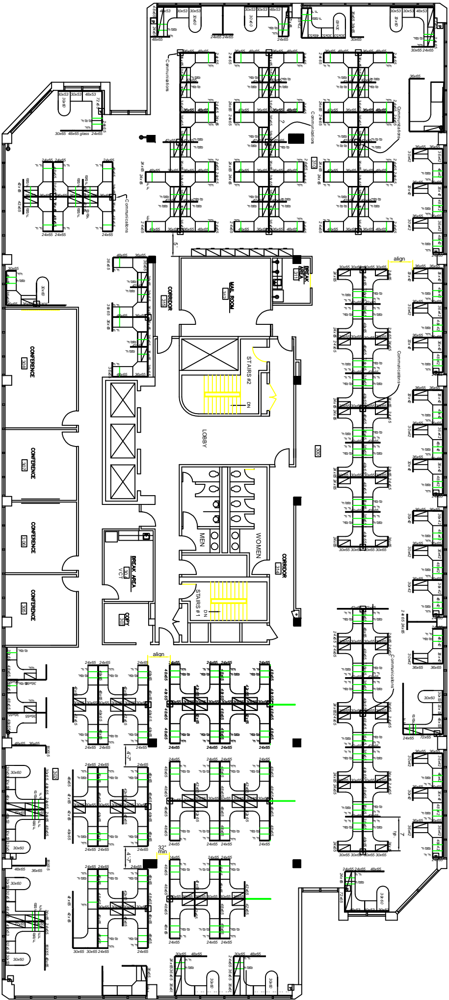
FURNITURE LOCATION PLAN SCALE 1/8"=1'-0"
